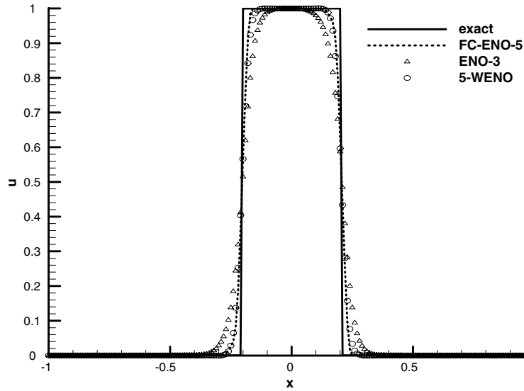
Fig. 4b. Numerical results of case 2, N = 200 , t = 6 .
