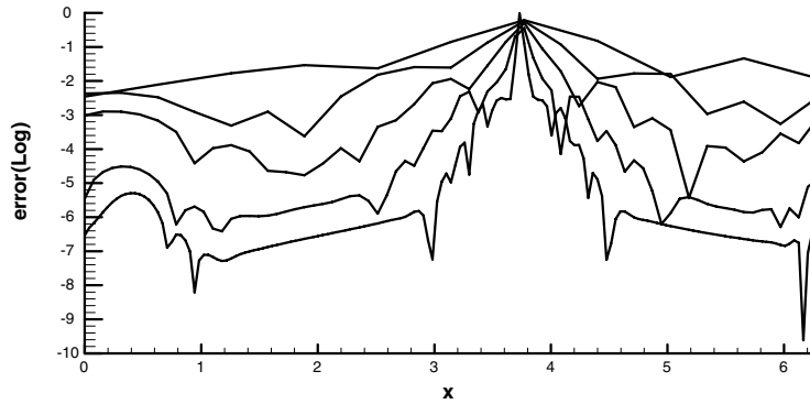
Fig. 6e. Point-wise errors of the FC-TVD scheme.
