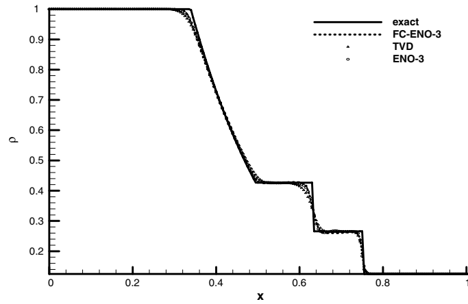
Fig. 8b. Comparisons of density of Sod problem.
