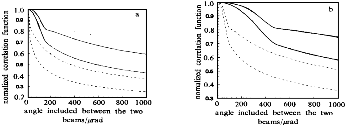
Fig. 3 Relationship between normalized correlation function of coefficients of Zernike polynomials and \theta The solid lines and the dashed lines are corresponding to R = 0.25\text{m} and R = 0.05\text{m} , respectively. (a) L = 3\text{km} , (b) L = 1\text{km}
