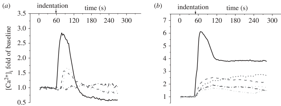
Figure 4. A set of typical [Ca^{2+}]_i transients of individual cells in the (a) linear and (b) hexagonal chain patterns. Roman number represents the position of a cell in the network as defined in figure 1. The calcium responses were recorded for approximately 5 min, 1 min for baseline and 4 min during AFM indentation. The [Ca^{2+}]_i concentration is represented by the cell image intensity normalized to the average value of baseline images. Solid lines, cell I; large dashed lines, cell II; small dashed lines, cell II'; dotted lines, cell III; dashed double dotted lines, cell III'; dashed dotted lines, cell IV.
