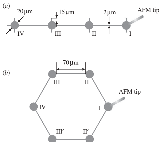
Figure 1. Schematic drawings of the designed (a) linear and (b) looped hexagonal chain patterns. One of the cells in the cell chain is mechanically stimulated by indenting on it with an atomic force microscope (AFM) tip.
