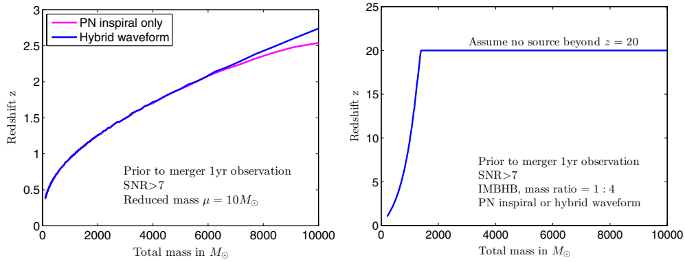
Figure 2. All-angle averaged detection range under a single Michelson threshold SNR of 7, with a prior to merger 1yr observation. Left: stellar mass black hole spiralling into IMBH with a reduced mass of 10M_{\odot} . Right: 1:4 mass ratio IMBH–IMBH binary.
