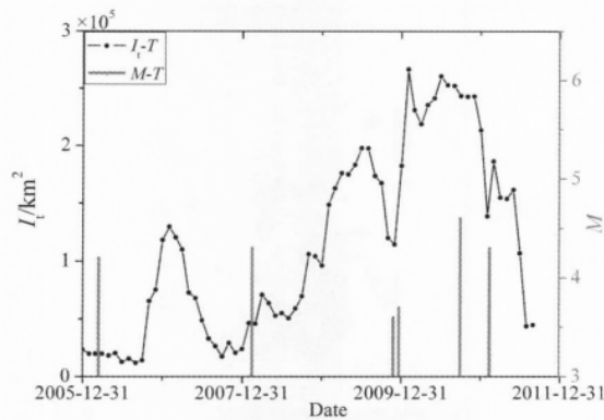
图7 周口地震异常区的 I_t 变化及地震时序 Fig. 7 I_t and the earthquake sequence in the seismogenic zone of Zhoukou earthquake
