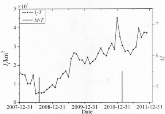
图9 阿勒泰地区异常区内 I_t 变化及地震时序 Fig. 9 I_t and the earthquake sequence in the seismogenic zone in Altay
