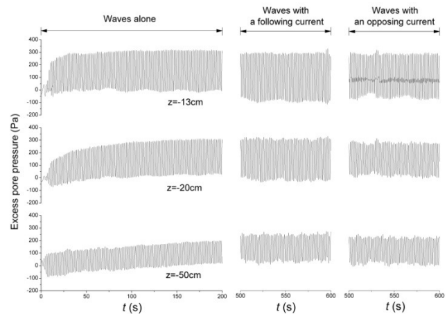
Fig. 7. Typical time series of pore pressure responses at various depth in the silty bed under conditions of waves alone, waves with a following current and waves with an opposing current from Test 3-1, 3-4 and 3-5 ( H_0 = 11.1\text{cm} , T = 1.6\text{s} , U_c = \pm 0.20\text{m/s} )
