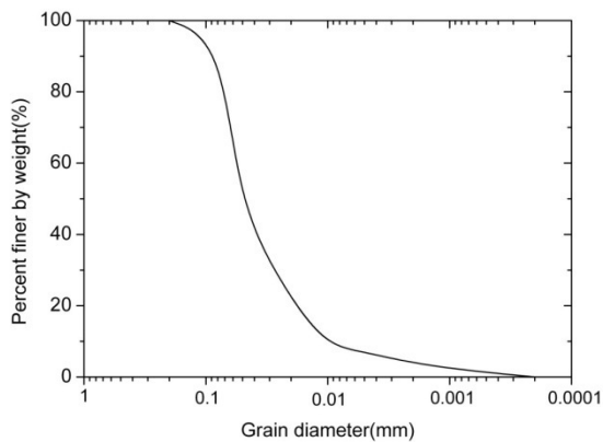
Fig. 2. Grain size distribution curves of the test silt
