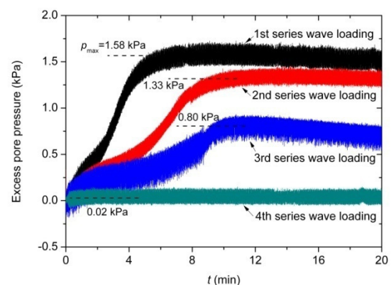
Fig. 3. Time series of excess pore pressure for different stages of wave loading at z = -50 cm ( H = 7 cm, T = 1.5 s)
