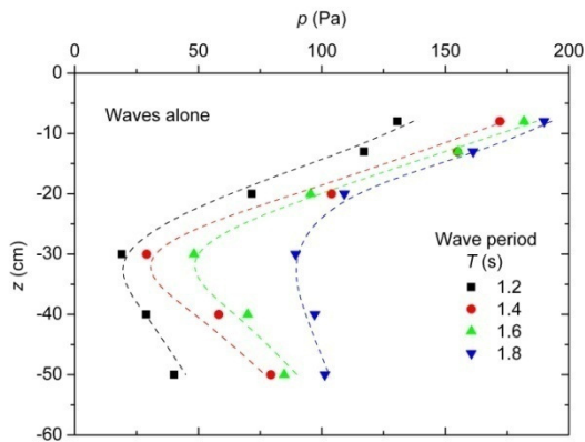
Fig. 4. Comparison of depth profiles of the pore pressure amplitudes under waves alone condition between different value of wave periods ( H = 11.0\text{cm} )
