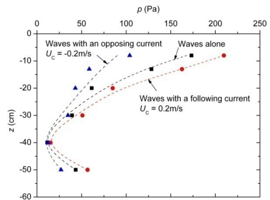
Fig. 8. Comparison of depth profiles of the pore pressure amplitudes between the cases of waves alone, waves with a following current and waves with an opposing current ( H_0 = 11.8\text{cm} , T = 1.2\text{s} )
