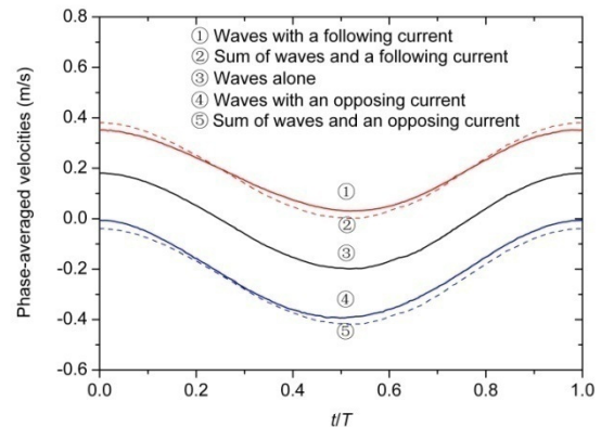
Fig. 6. Comparison of flow velocity variation over one cycle
