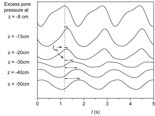
Fig. 5. Close-up picture of the excess pore pressure at various depth in the silty bed under waves alone condition from Test 3-1
