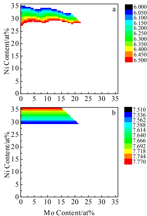
Fig.2 Criterion surface graphs after primary screening: (a) X_{\text{Allen}} and (b) VEC
