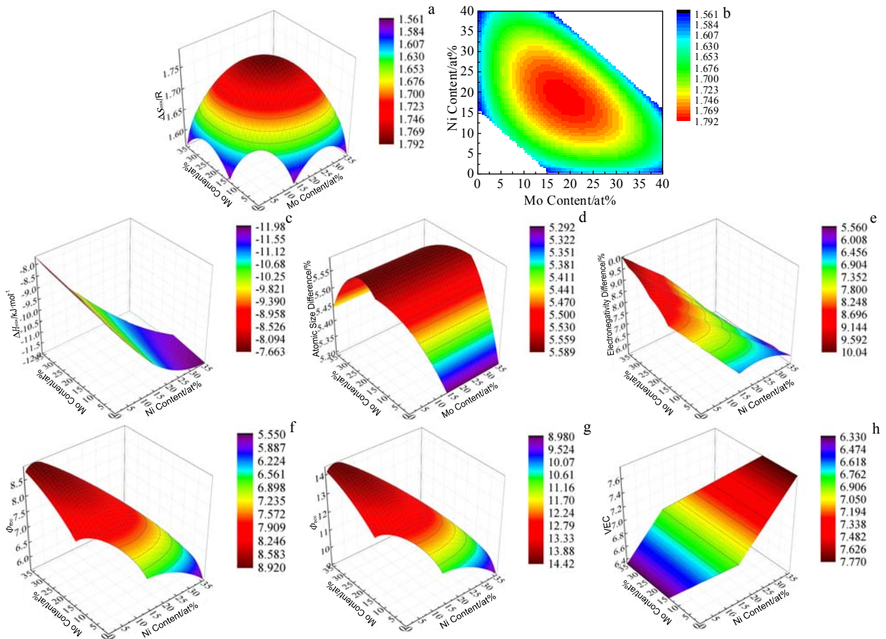
Fig.1 Surface graphs of different criteria: (a, b) \Delta S_{mix} , (c) \Delta H_{mix} , (d) \delta , (e) X_{Allen} , (f) \Phi_{fcc}(\xi=0.74) , (g) \Phi_{bcc}(\xi=0.68) , and (h) VEC
