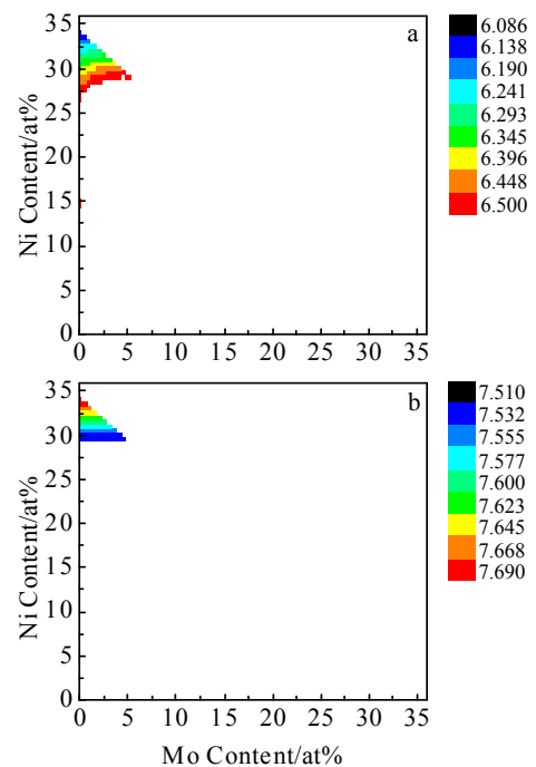
Fig.3 Criterion surface graphs: (a) X_{\text{Allen}} and (b) VEC
