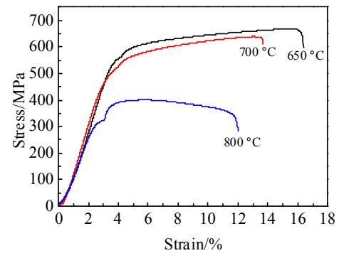
Fig.10 High temperature tensile stress-strain curve of the as-cast AlCoCrFeMo 0.05 Ni 2 high entropy alloy
